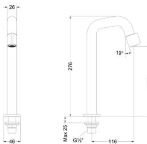
Pact contour L Pact deck mounted contour L
