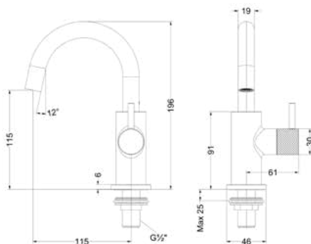
Nexus met draaibare uitloop Nexus deck mounted with swivel spout
