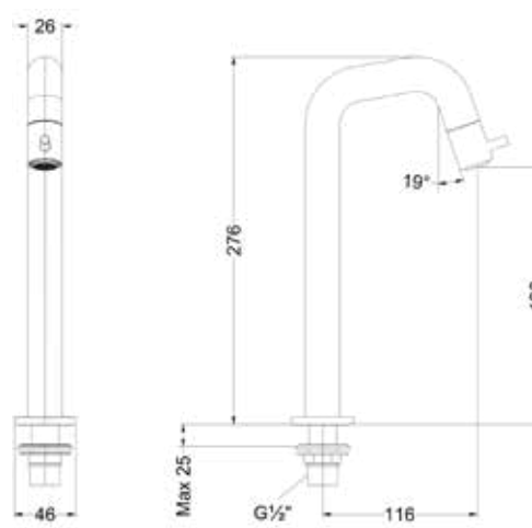
Bond contour L
