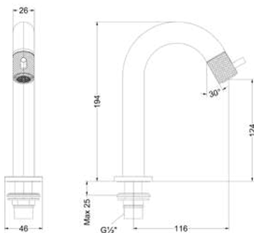
Nexus stand gebogen S Nexus deck mounted curved S
