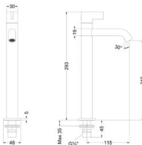
Pact stand L Pact deck mounted L
