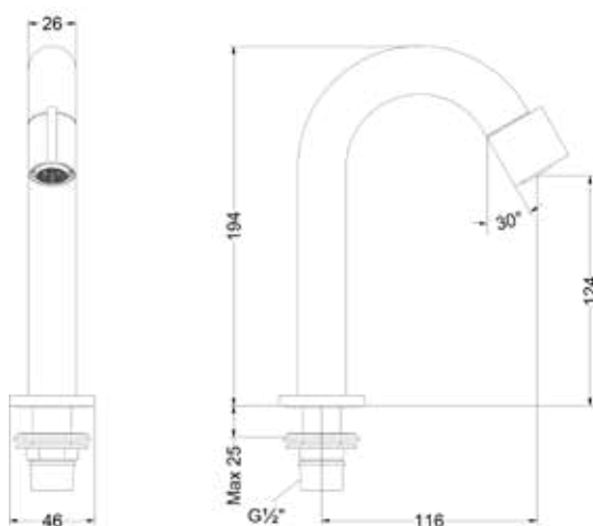
Pact stand gebogen S Pact deck mounted curved S
