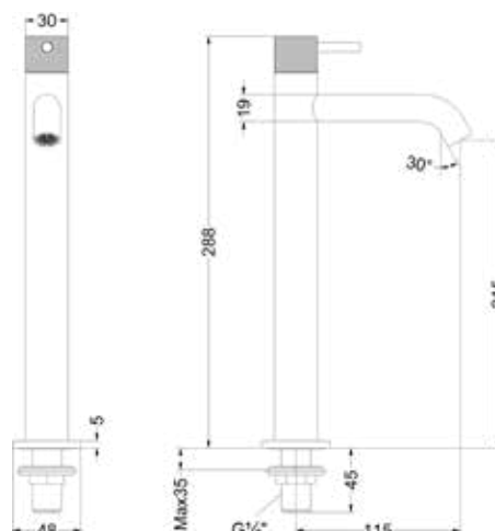
Nexus stand L Nexus deck mounted L
