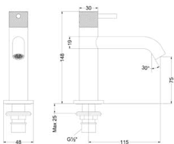
Nexus stand S Nexus deck mounted S
