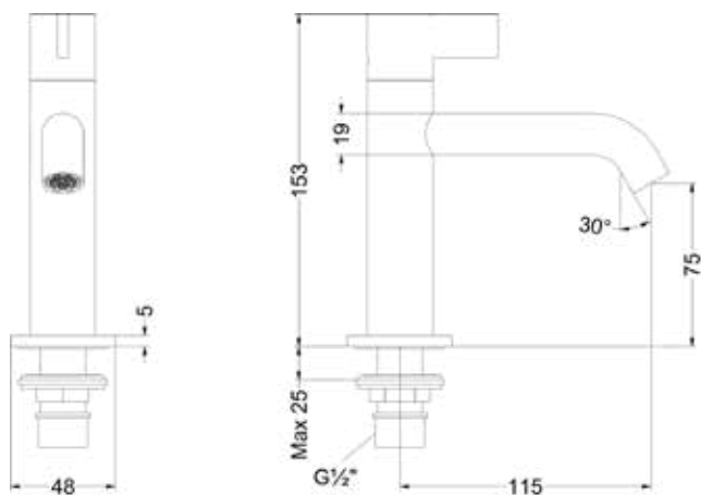
Pact stand S Pact deck mounted S
