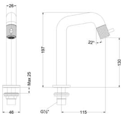
Nexus contour S Nexus deck mounted contour S
